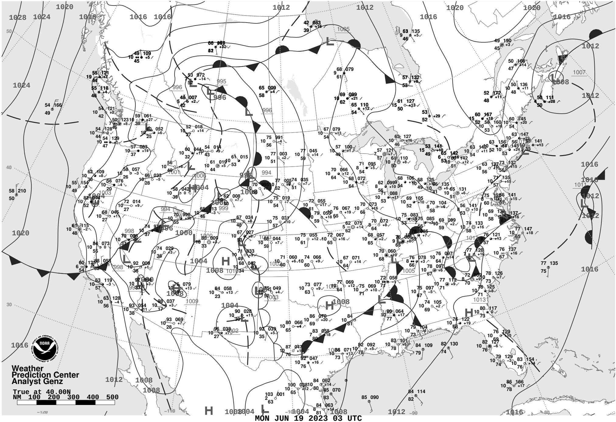
Surface Weather Map and Station Weather
