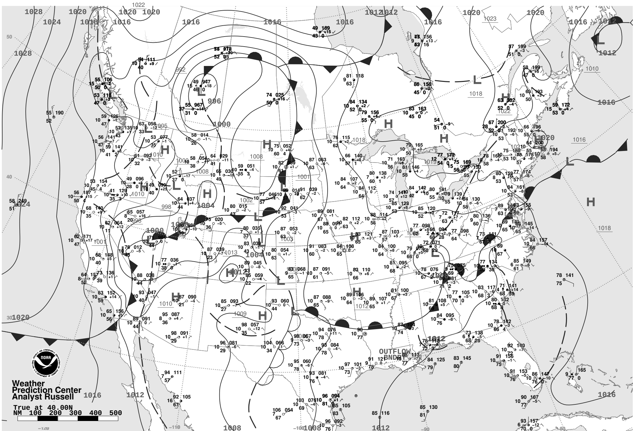
MON JUN 19 2023 18 UTC Surface Weather Map and Station Weather
